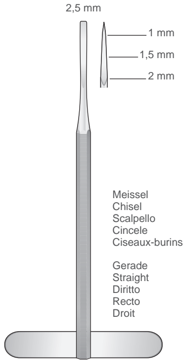
51-450-01 130 mm
