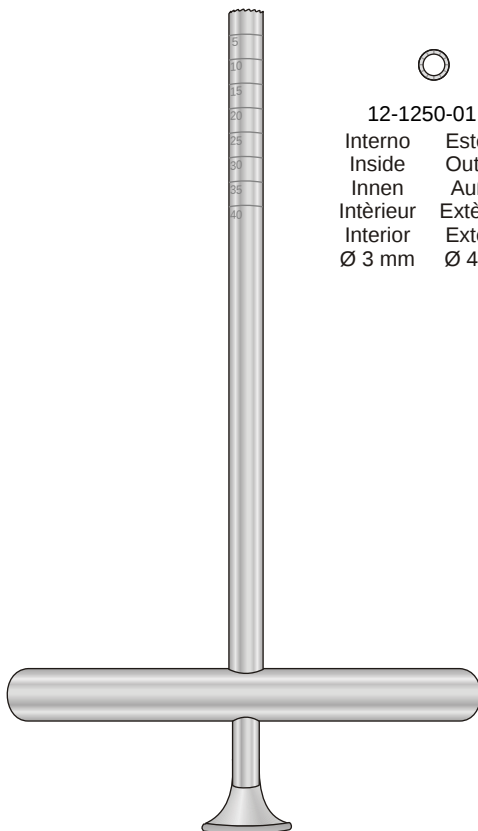
12-1250 170 mm
